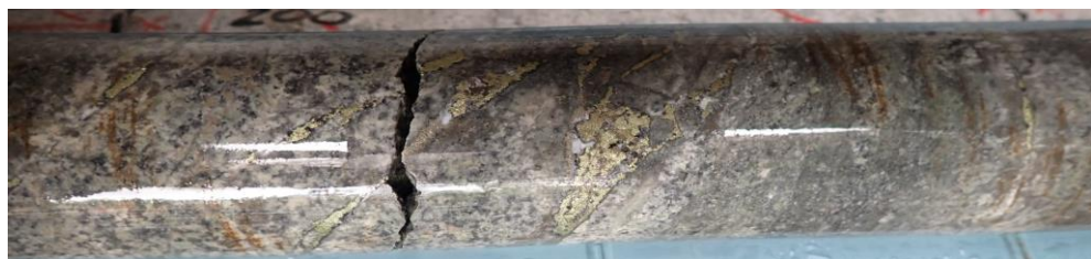
Figure 1 – Example of chalcopyrite vein mineralisation in drill hole BRURD002 (201.1 – 201.3m)
