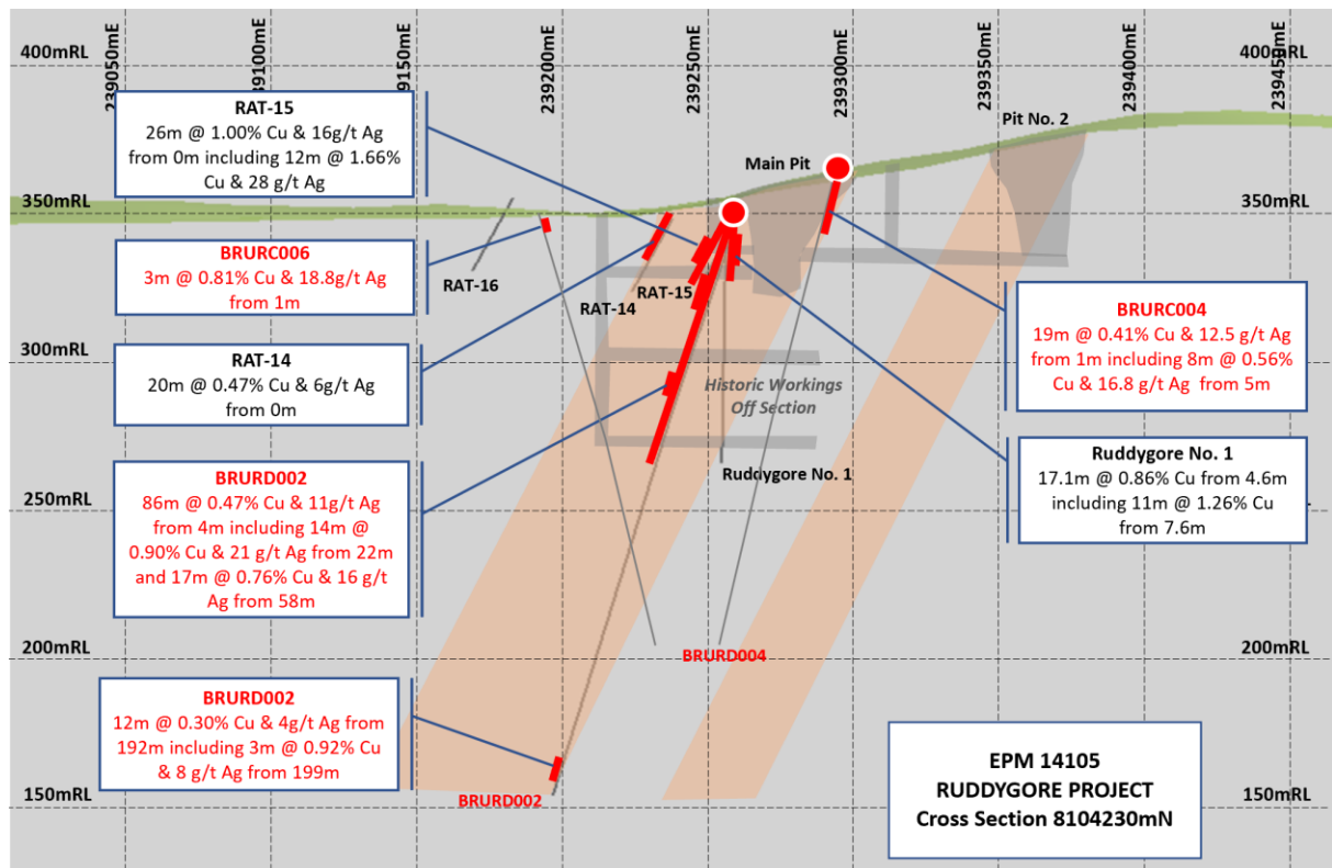
Figure 4 – Cross section looking north at Ruddygore drill hole BRURD002 and other historic drill holes located north of the historic Ruddygore mine
