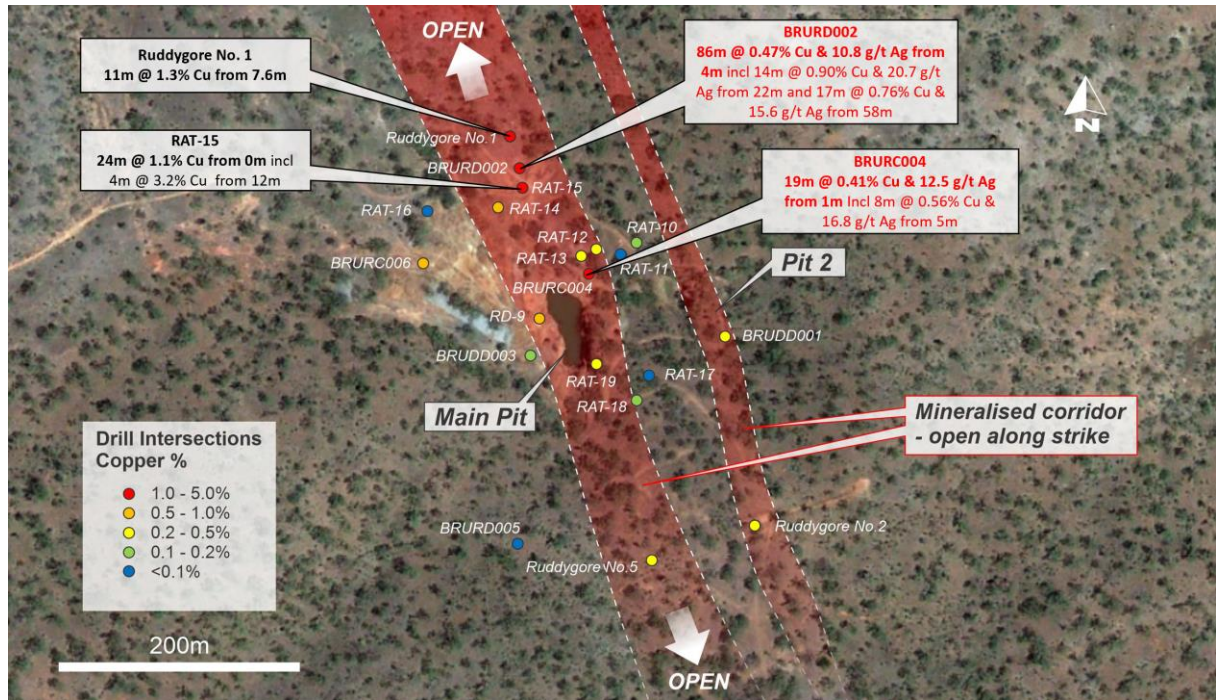
Figure 3 – Plan view of Ruddygore area with drill hole collar locations coloured by copper grade and the location of interpreted copper-mineralised corridors.
