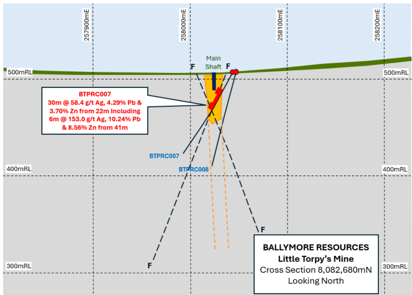
Figure 2 – Torpy's Cross Section 8,082,680mN looking north, showing historic workings, drill traces massive sulphide lenses.
