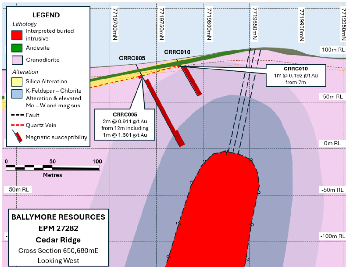
Figure 4 – Cross section 650,680mE looking west at the Cedar Ridge Prospect.
