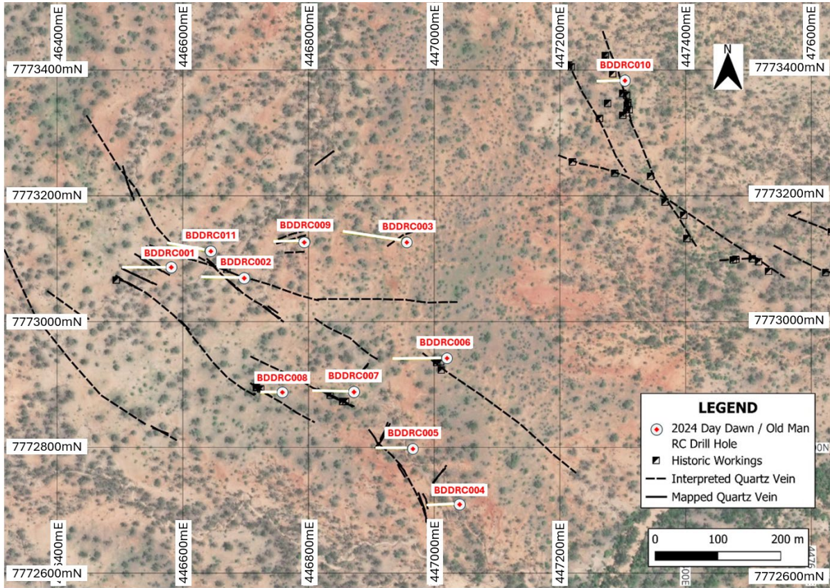
Figure 5 – Day Dawn drill hole locations.
