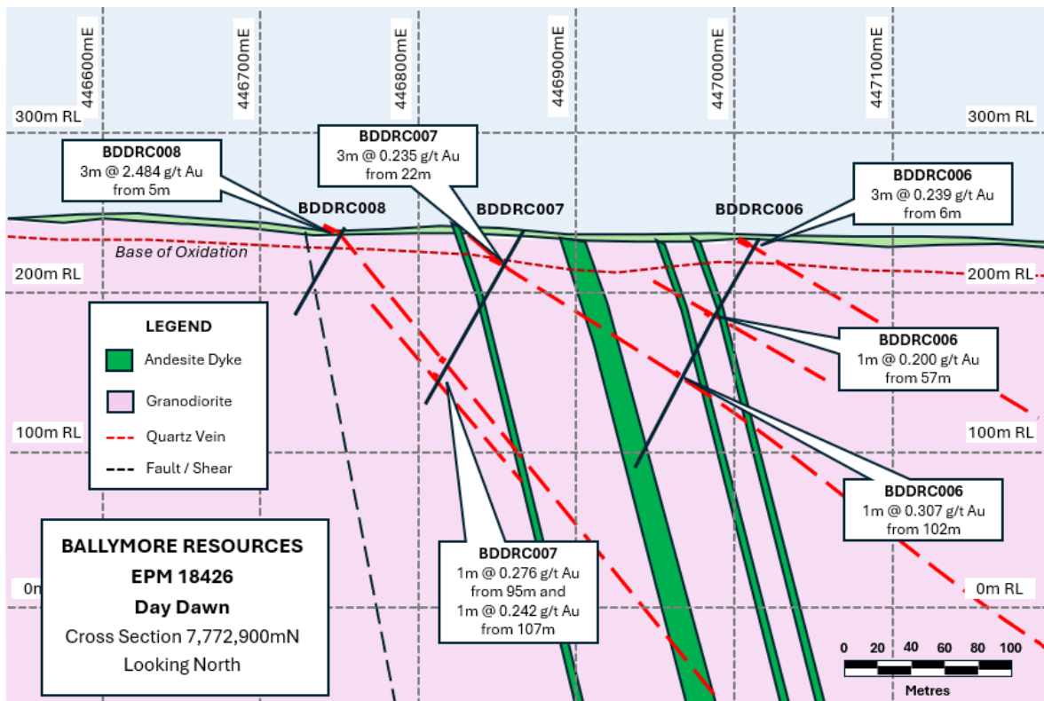
Figure 6 – Cross section 7,772,900mN looking north at the Day Dawn Prospect.
